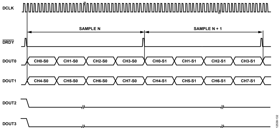
Figure 117. FORMAT0 = 0, FORMAT1 = 1 —Channel 0 to Channel 3 Share DOUT0 , and Channel 4 to Channel 7 Share DOUT1 (S0 Means Sample 0 and S1 Means Sample 1)
