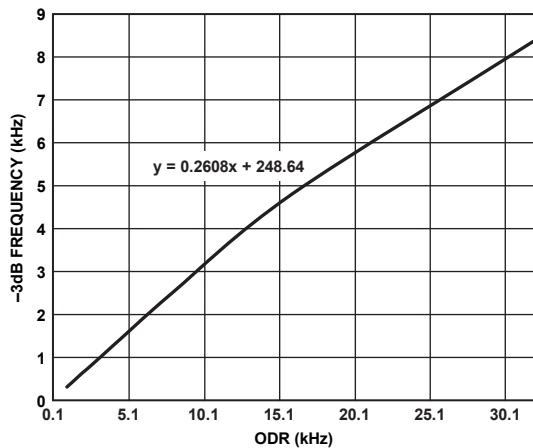
Figure 112. -3 dB Correction Factor
