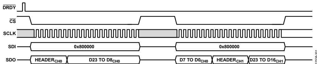
Figure 105. SPI Used to Read Back the Σ-Δ ADC Data, in 24-Bit Frames
