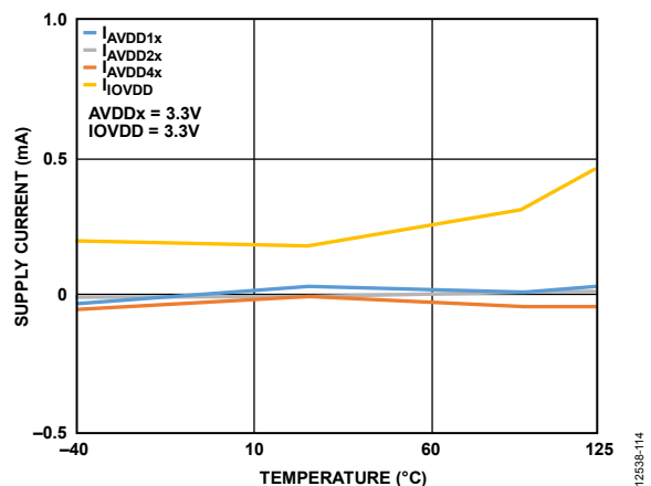
Figure 97. Shutdown Current
