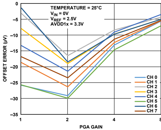
Figure 40. Offset Error vs. PGA Gain, High Resolution Mode
