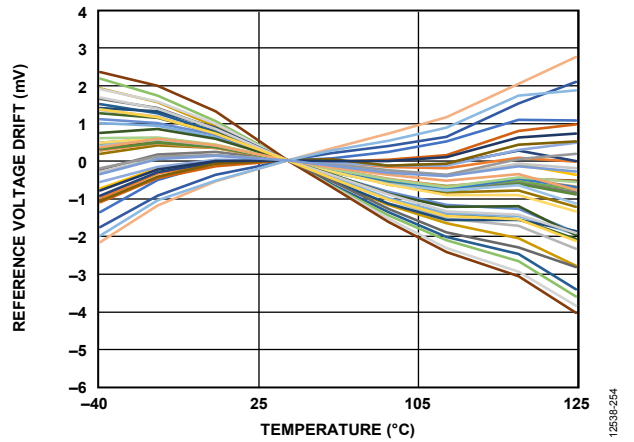
Figure 54. Internal Reference Voltage Drift
