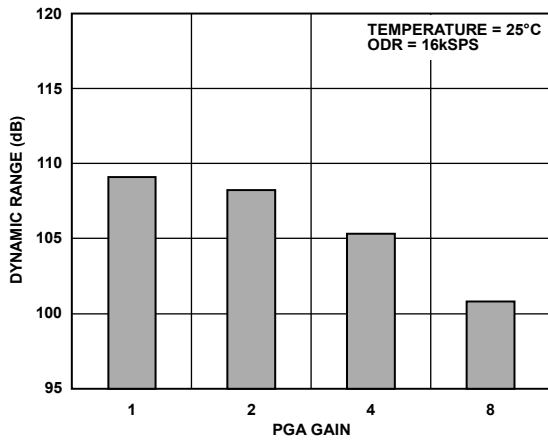
Figure 39. Dynamic Range vs. PGA Gain, High Resolution Mode
