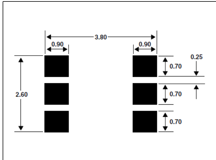
Figure 39: Suggested TMB-6 Package PCB Layout
