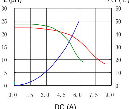
11. CDRH127L125NP-680MC
