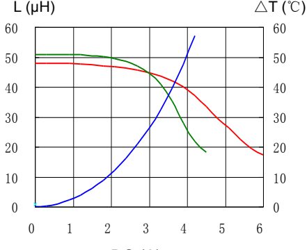
10. CDRH127L125NP-470MC
