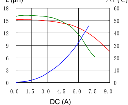
10. CDRH127L125NP-470MC
