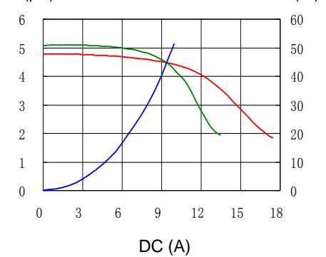
6. CDRH127L125NP-100MC
