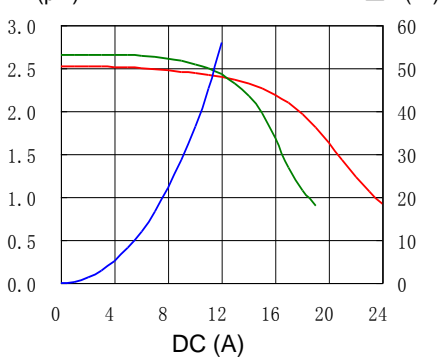
4. CDRH127L125NP-6R2NC
