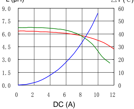
7. CDRH127L125NP-150MC
