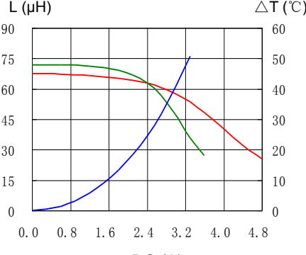
11. CDRH127L125NP-680MC
