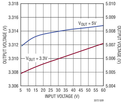
Output Voltage Line Regulation Forced Continuous Mode
