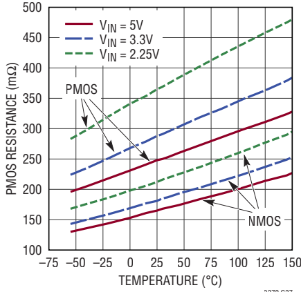
1A Buck NMOS and PMOS R_{DS(ON)} vs Temperature Across V_{IN}
