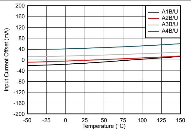
Figure 7-2. TMCS1107 Input Offset Current vs. Temperature
