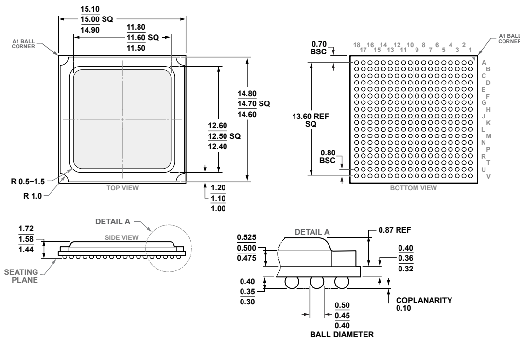
Figure 100. 324-Ball Ball Grid Array, Thermally Enhanced [BGA_ED] (BP-324-3) Dimensions shown in millimeters
