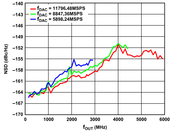
Figure 29. Single-Tone NSD Measured at 10% Offset from f_{OUT} vs. f_{OUT} over f_{DAC} , Shuffle On, 12-Bit Resolution, Mode 24C
