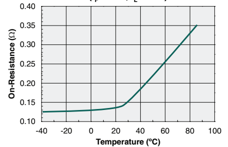
Typical On-Resistance vs. Temperature ( I_F=2mA , I_L=0.5A )
