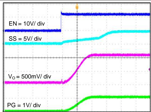
Figure 29. TPS562210A Start Up Relative To En
