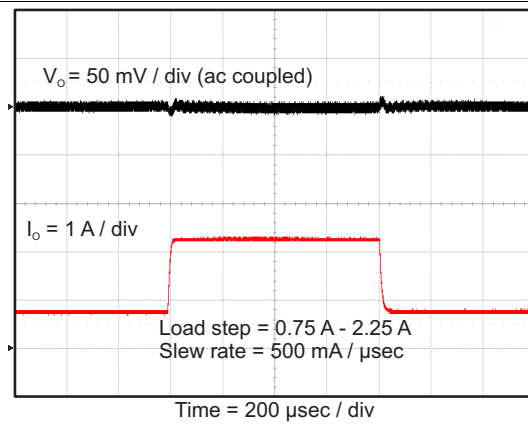
Figure 42. TPS563210A Transient Response
