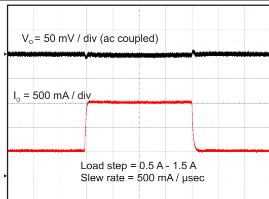
Figure 27. TPS562210A Transient Response
