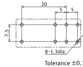
Recommended PC board pattern (BOTTOM VIEW)
